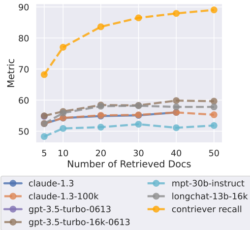
Figure 11: Retriever recall and model performance as a function of the number of retrieved documents. Model performance saturates long before retriever recall , indicating that the models have difficulty making use of the extra retrieved documents.
